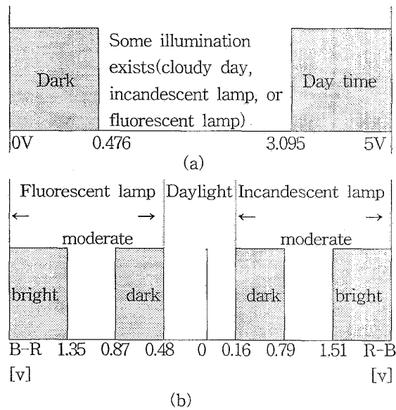
Fig. 5. Decision function. (a) Intensity decision function(G-sensor) (b) Outer illumination decision function.
