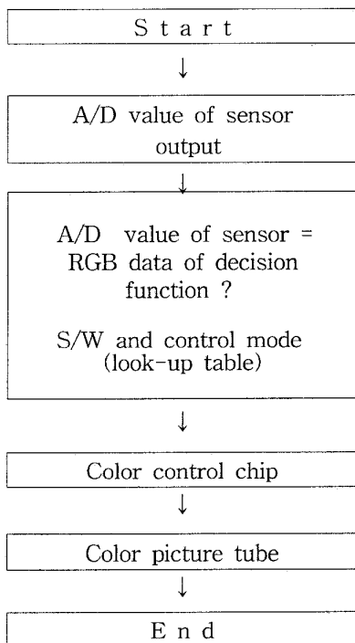
Fig. 6. Block diagram for color enhancement.
